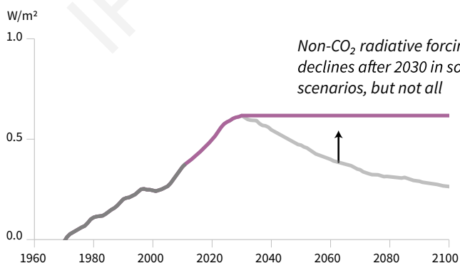
d) Scenarios for non-CO 2 radiative forcing
